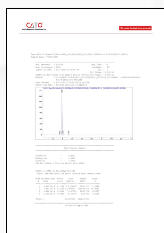
HPLC
